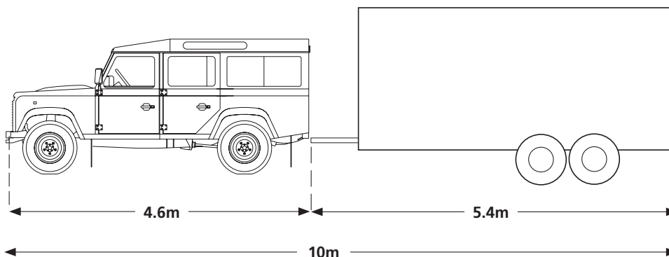
VEHICLE/TRAILER SIDE VIEW:
