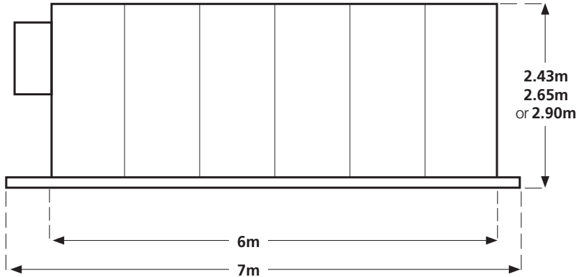
WALL UPRIGHT FRONT VIEW:
