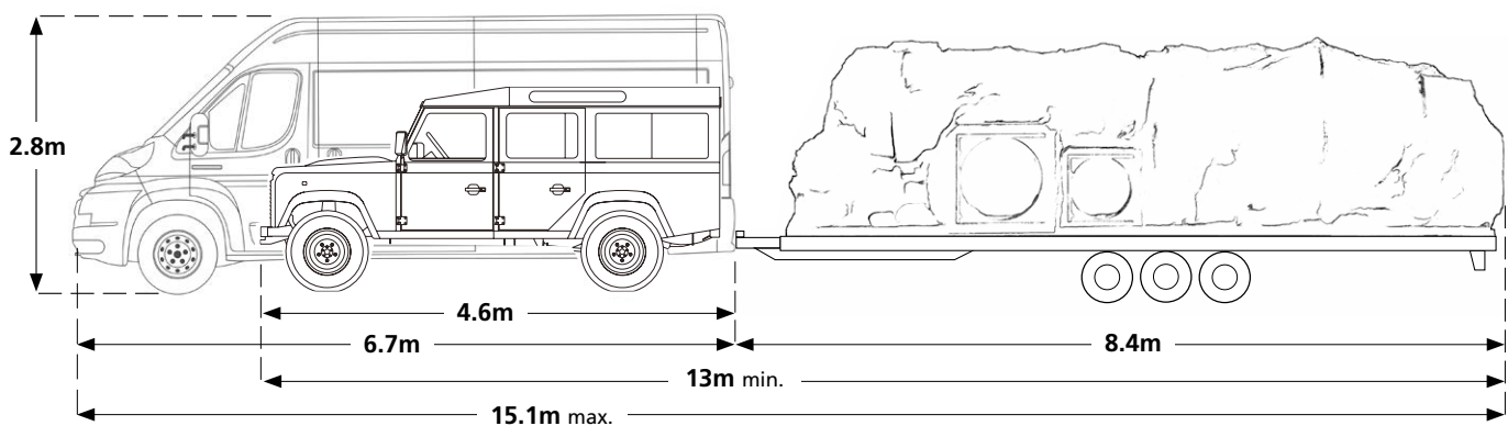
VEHICLE/CAVE SIDE VIEW:
