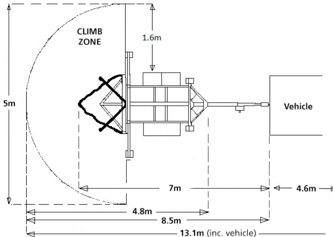
WALL UPRIGHT BIRDS-EYE VIEW:
