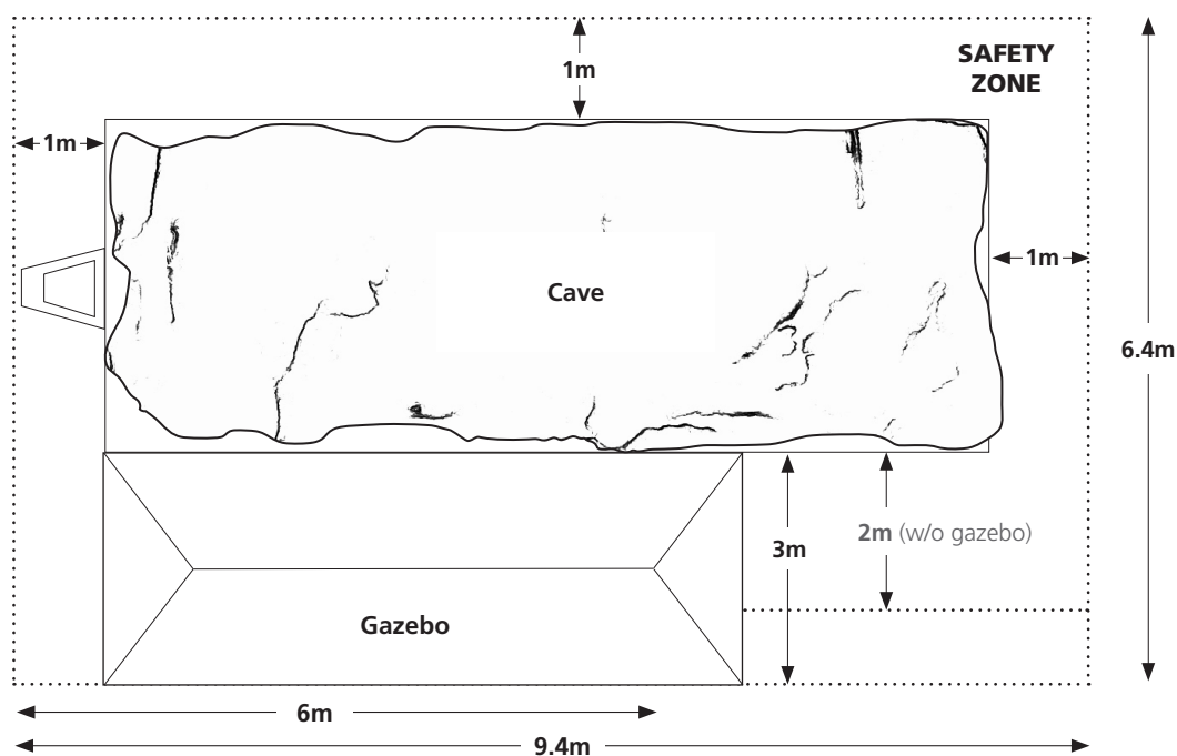
CAVE/GAZEBO BIRDS-EYE VIEW: (RECOMMENDED LAYOUT)
